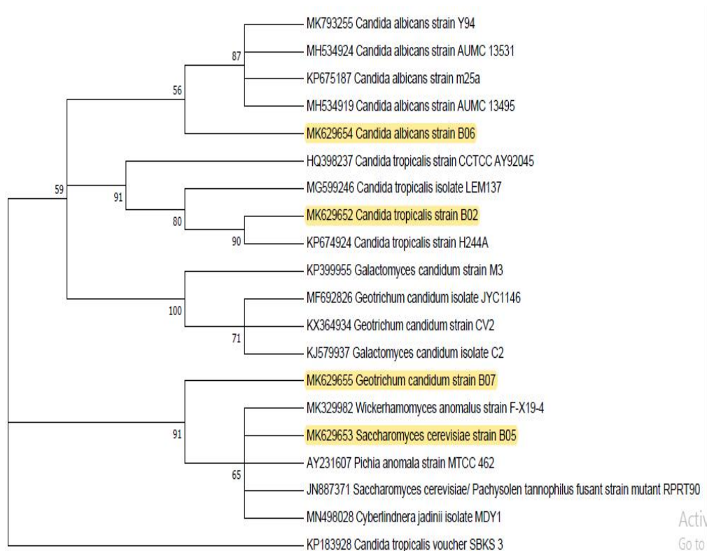
Figure 1: Evolutionary relationship of Yeast isolates sample
