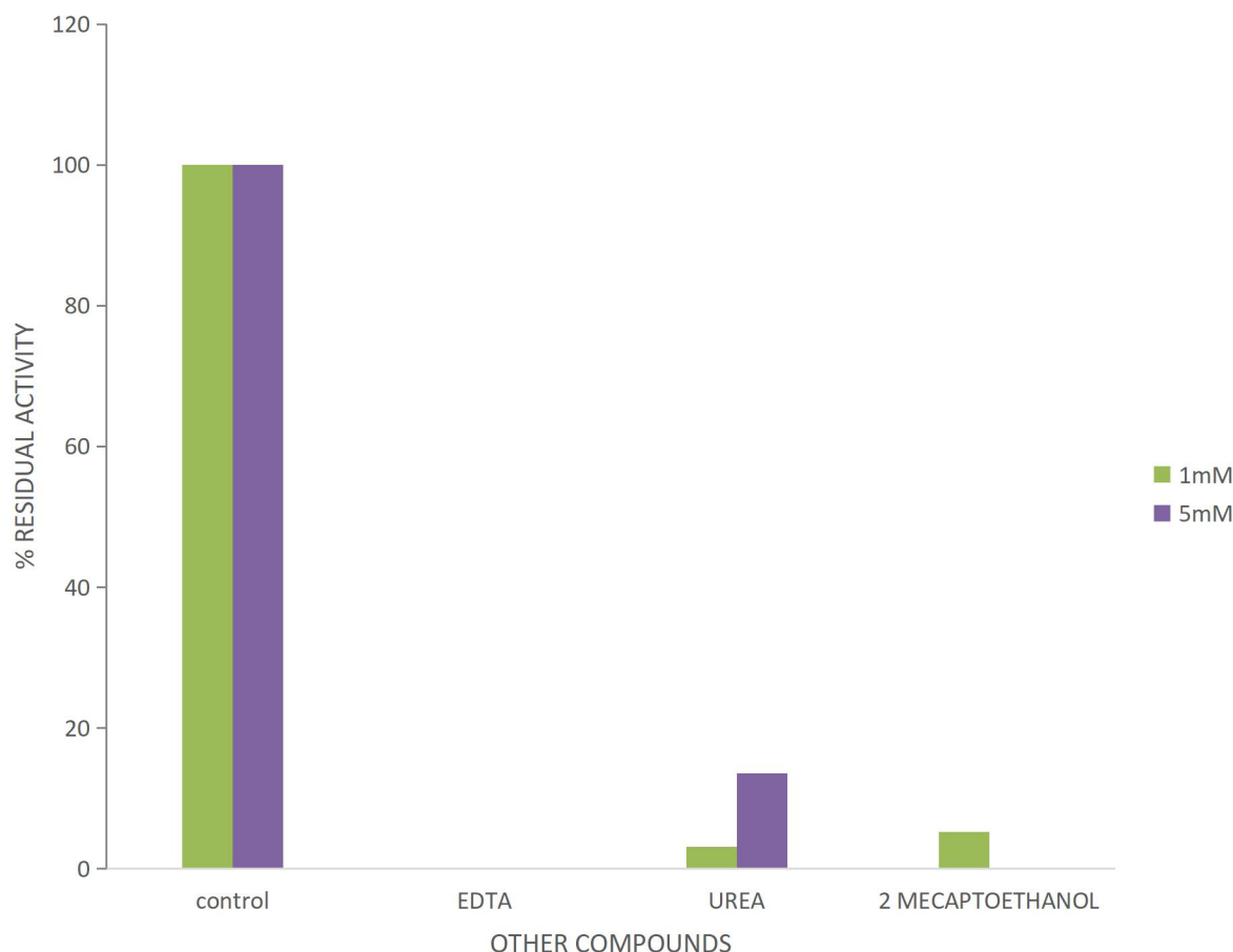
Figure 5: Effect of other compounds on phytase activity
